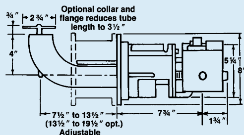
Dimensions HU Left Side
